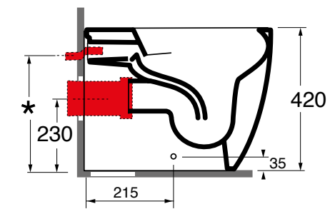
OCER/DP Raccordo eccentrico per entrata acqua H345 / H375 mm. Eccentric joint for water inlet - H345 mm / H375mm.
