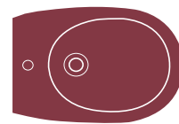
OVV Bidet a terra filo muro Floor mounted bidet back to wall 52 x 35,5 x h42
