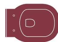
CLAW54 Vaso a terra Floor mounted wc 54 x 39 x h40
